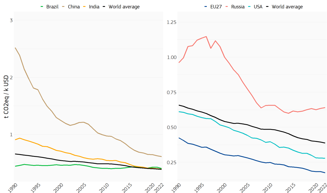
Figure 5. GHG emissions per unit of GDP PPP in top emitting economies, 1990-2022, (t CO 2eq /k USD) 29
