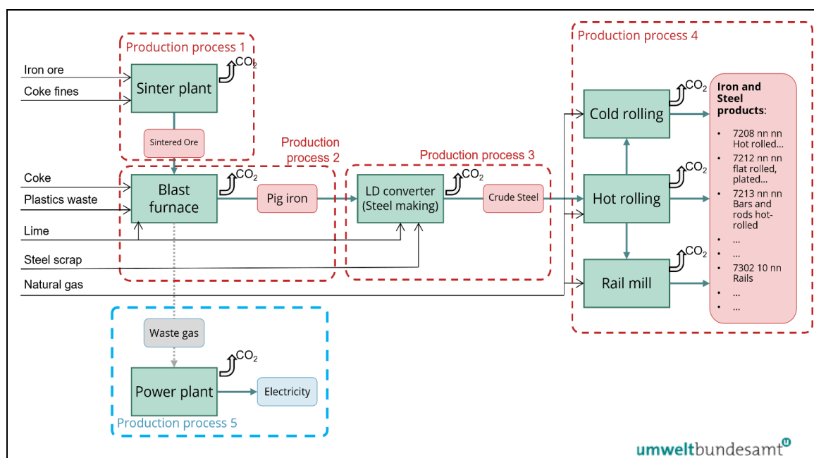
Figure 7-5: Example for carbon steel production, blast furnace route – Direct emissions and related source streams
