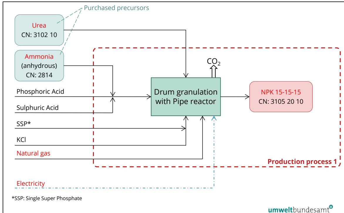
Figure 7-12: Fertilizer example – Overview and complete monitoring approach for the production of a mixed fertilizer grade.
