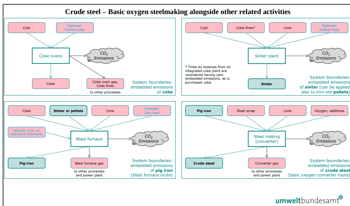
Figure 5-11: System boundaries of basic oxygen steelmaking and related processes.
